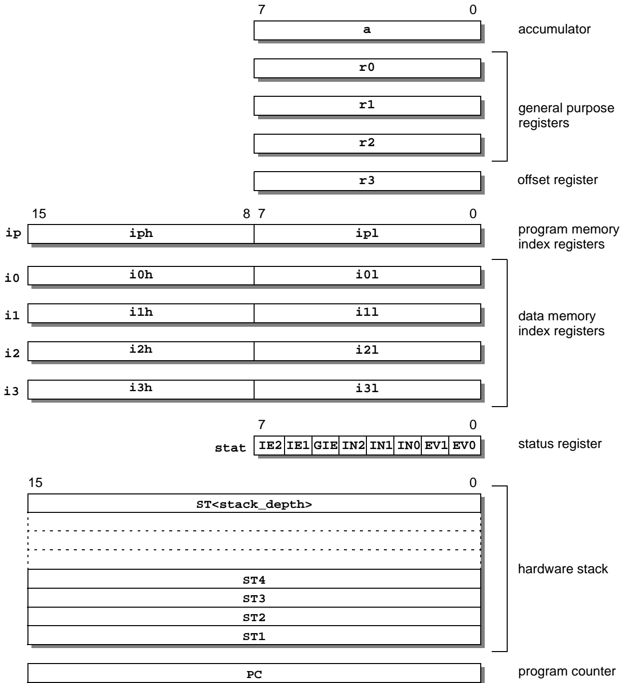
FIGURE 1.6: CR816DL registers.
