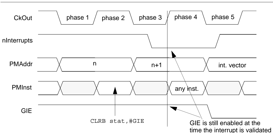
FIGURE 4.5: Interrupt disabling timing.
