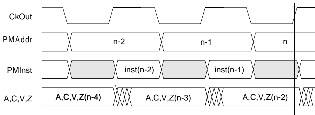
FIGURE 5.3: Pipeline snapshot.
