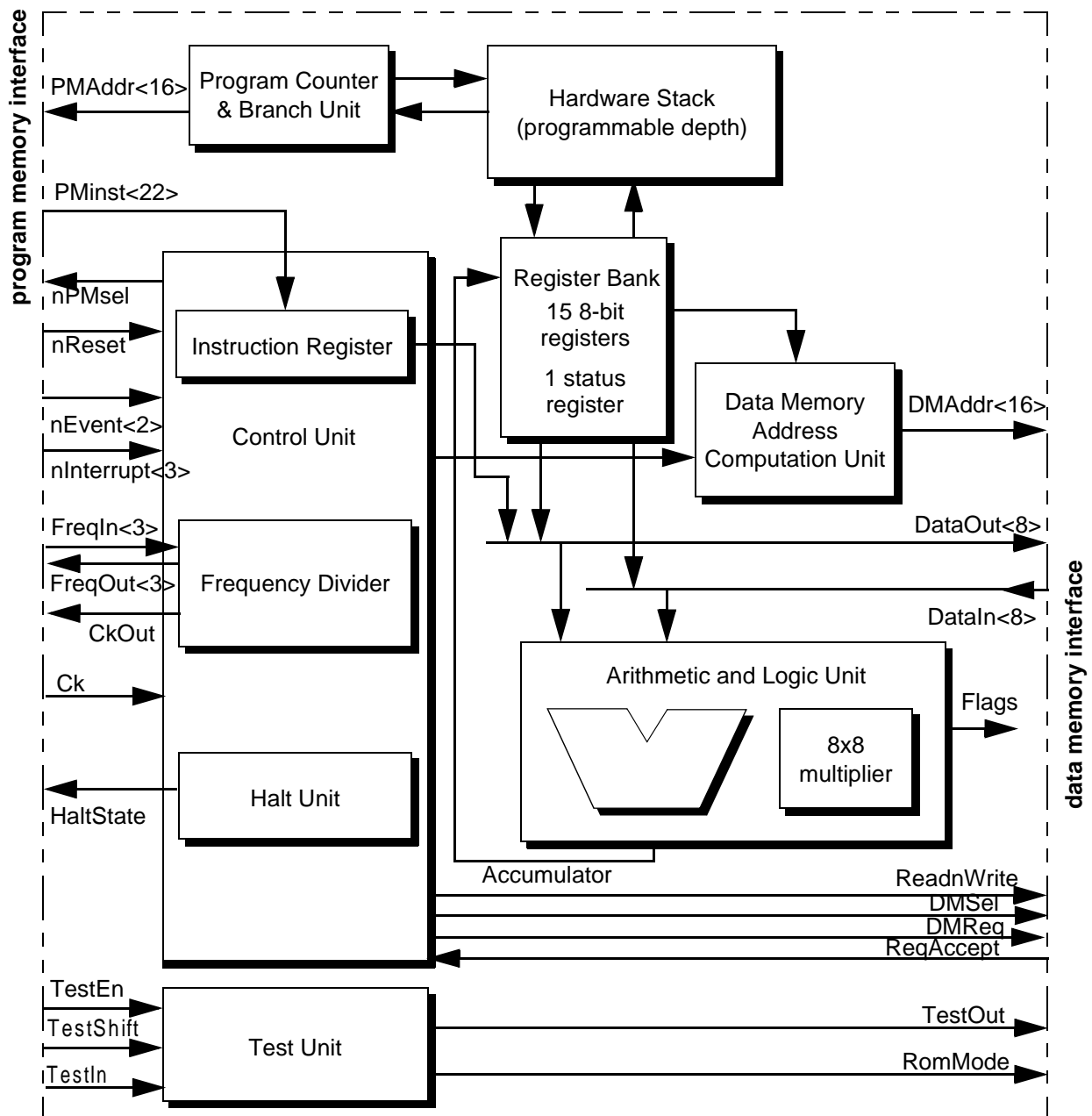
FIGURE 1.1: CR816 core diagram.
